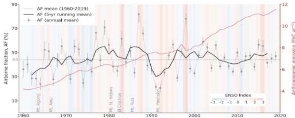
IPCC AR6
